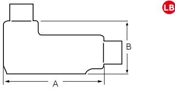
LB Form 7 Ferrous conduit bodies with covers
