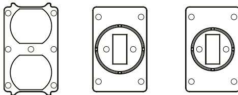
Single-gang (CKPM) – dimensions
