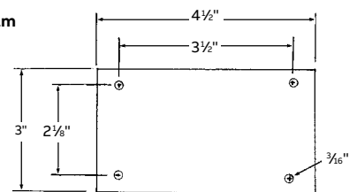
Plate dimensions
